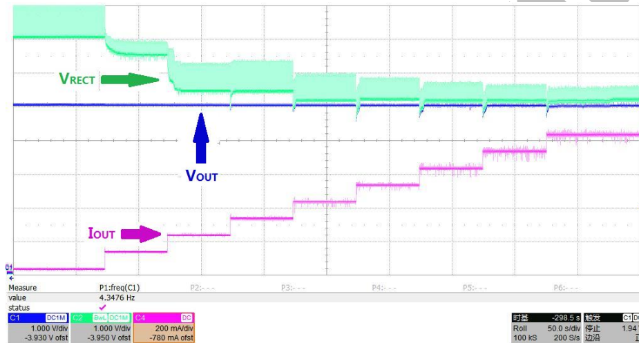
Figure8. V_{RECT} vs. V_{OUT} vs. I_{OUT}
